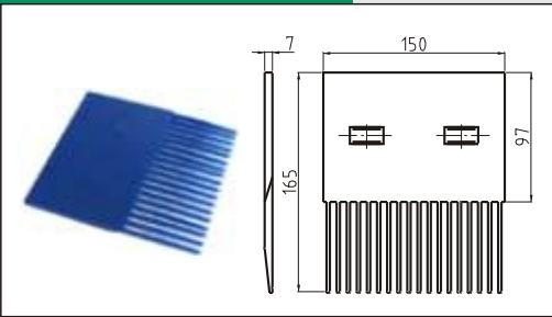
H900 Finger transfer plates 165X18T
