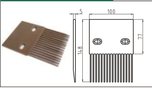
H100T16 Finger transfer plates 148X16T
