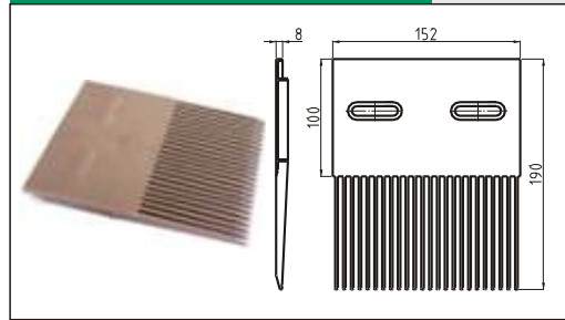
H3110T24 Finger transfer plates 190X24T
