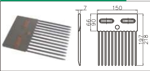
H4707ST12-2 Finger transfer plates 218X12T
