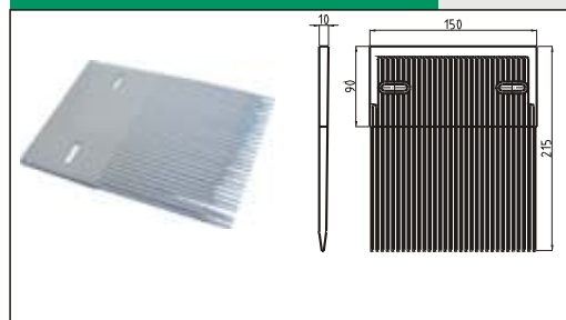
H2037T28 Finger transfer plates 215X28T
