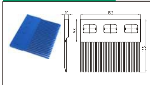
H2004T24 Finger transfer plates 135X24T
