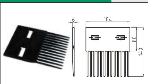
H5937T15 Finger transfer plates 148X15T
